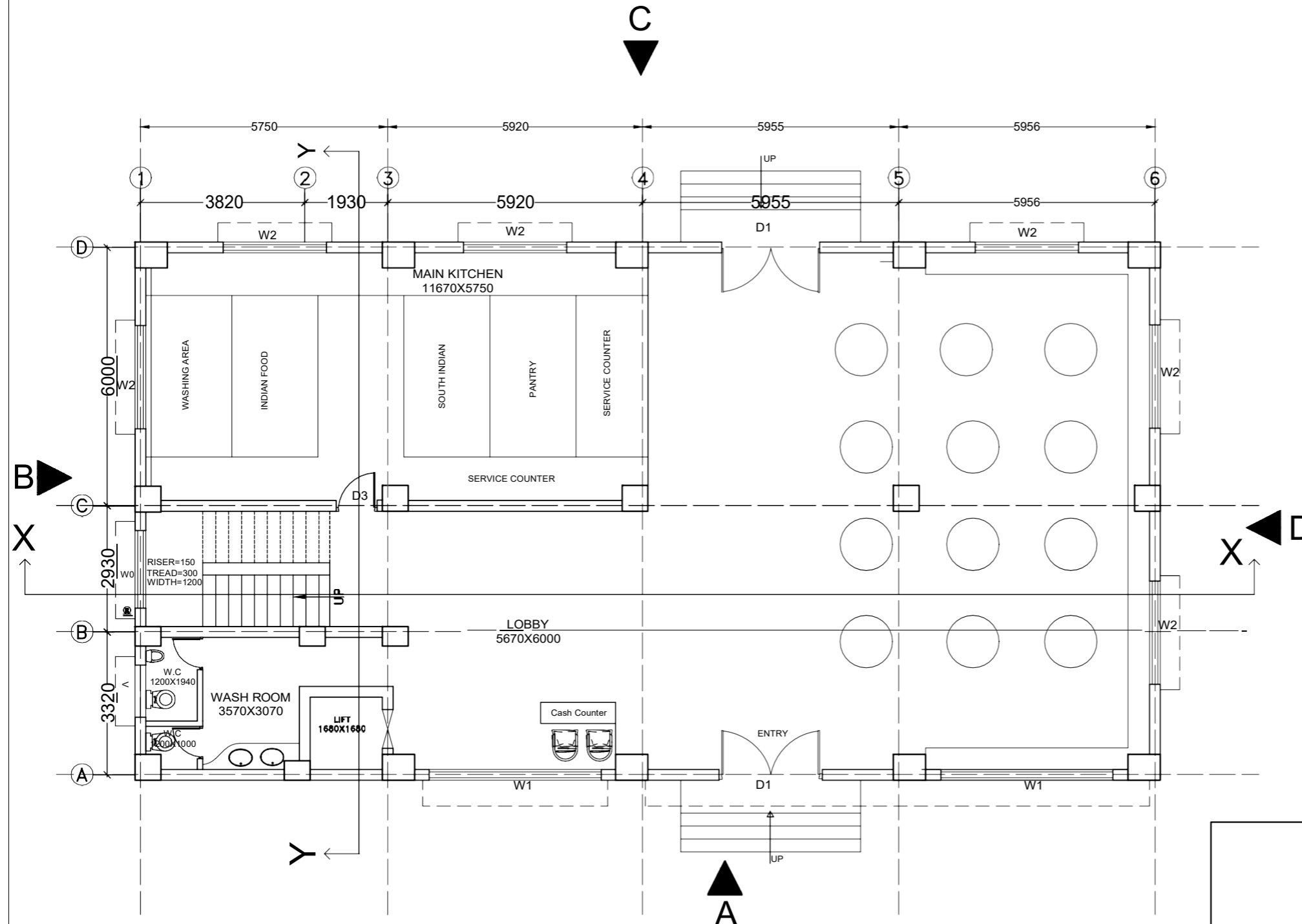
GROUND FLOOR PLAN: EATERY FOR COMMON MASSES
